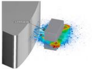
Magnetic flux evaluated from surface integral
