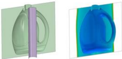
Wall thicknesses and temperature distributions when blow molding plastic containers [19.1]
